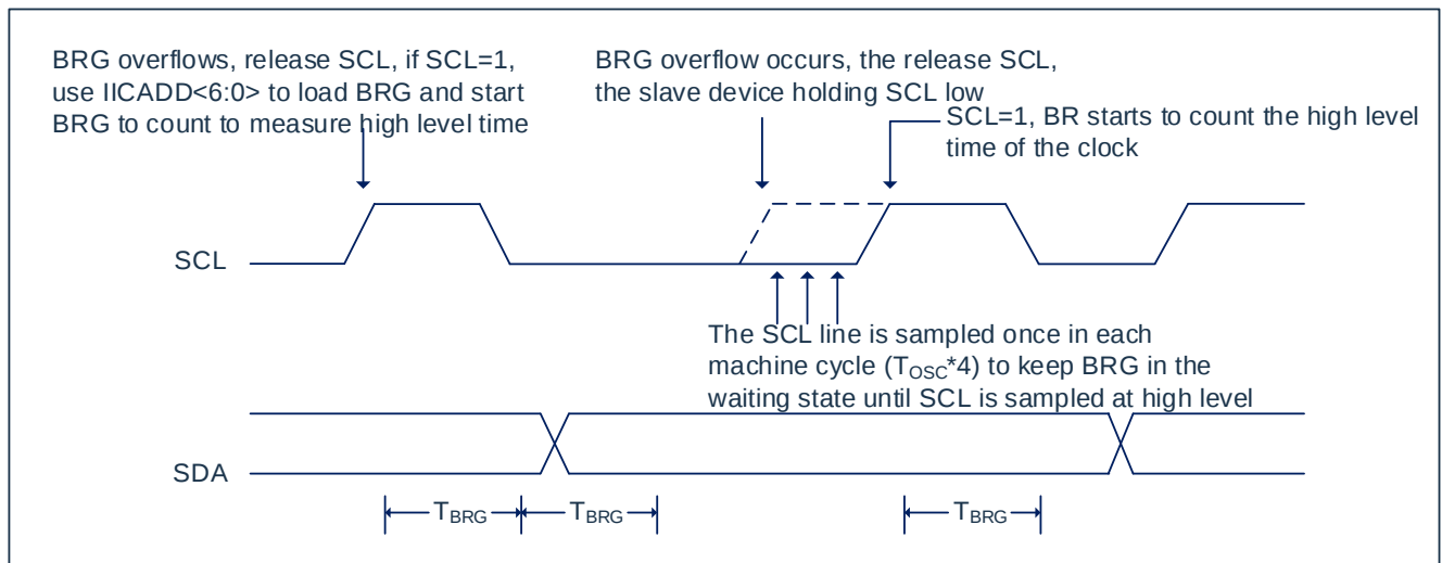
Fig 20-11: clock arbitration in master control transmit mode
