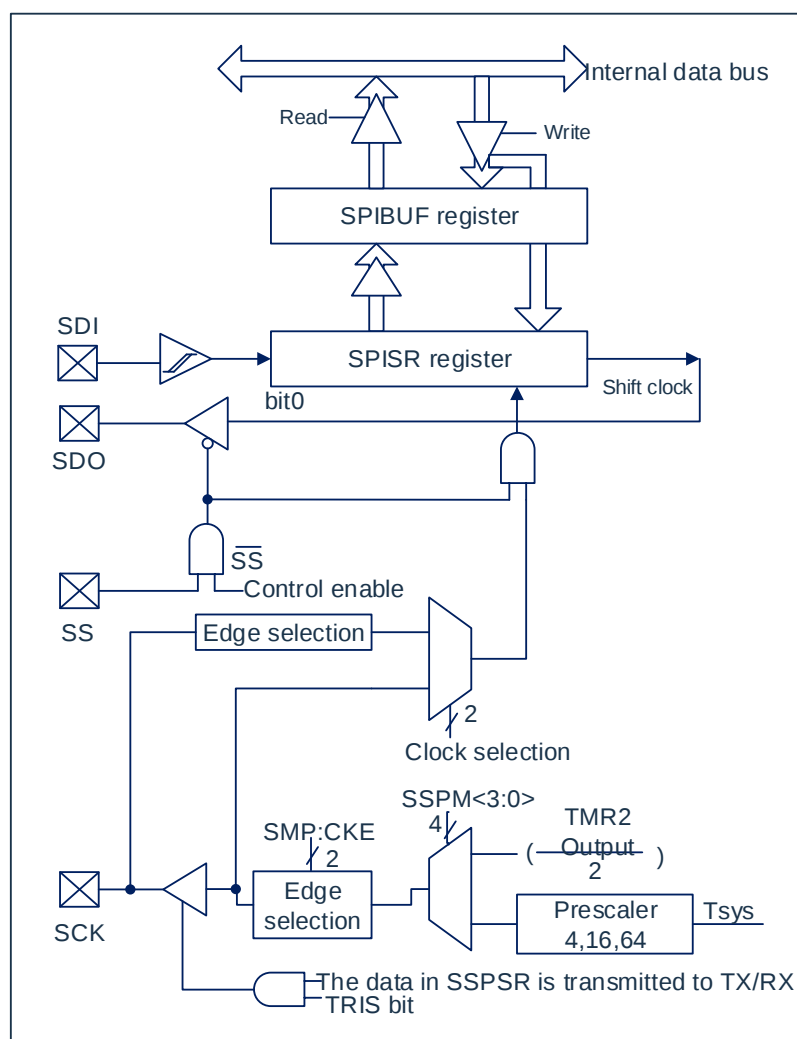
Fig 19-1 SPI mod block diagram
