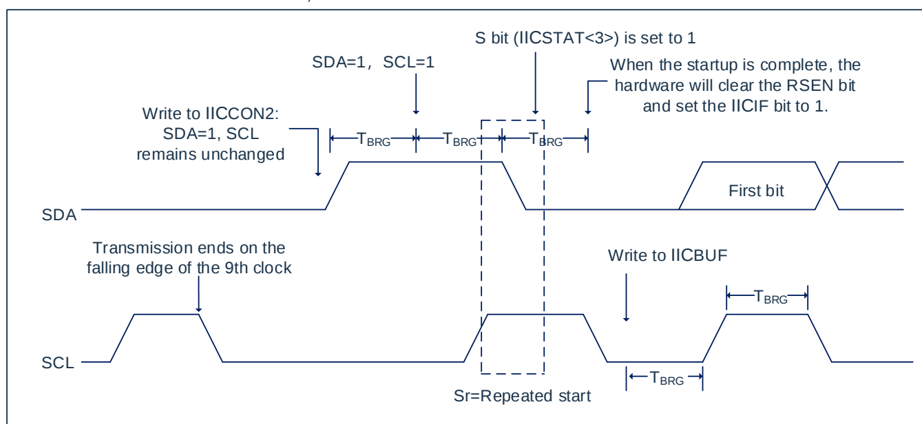
Fig 20-8: time series of repeat condition
